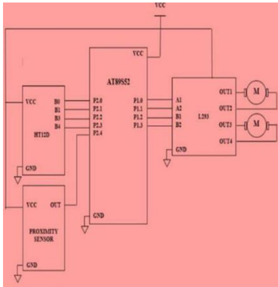
Fig. 4.4. Receiver circuit diagram
