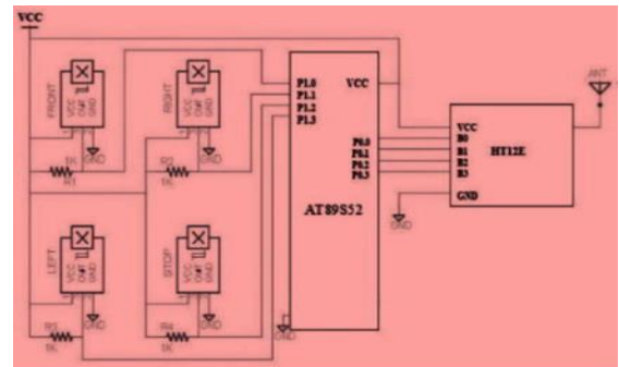
Fig.4.3. Transmitter circuit diagram
