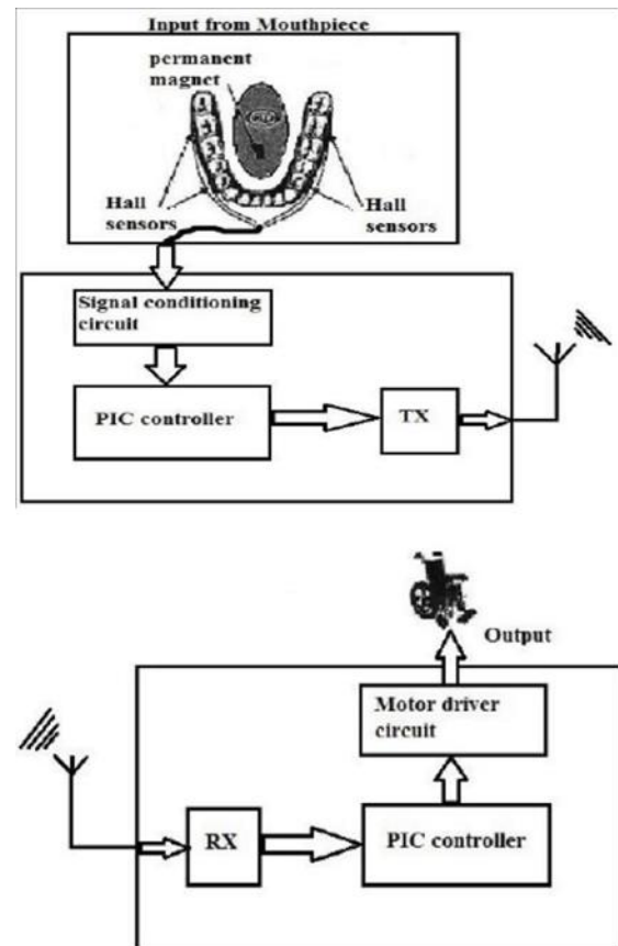
Fig.3.1. Simplified block diagram of the Tongue Drive system
