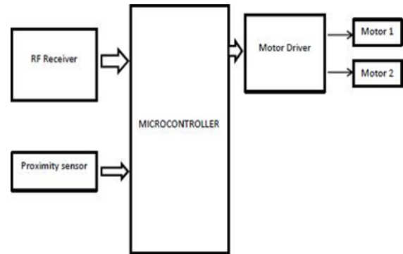
Fig.4.2. Receiver block diagram
